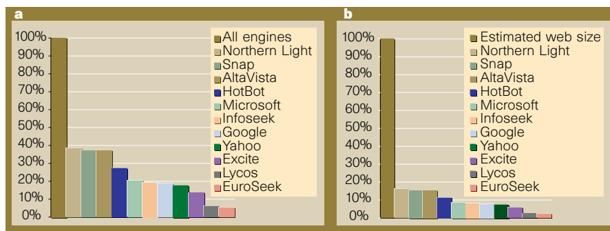
Figure 2 Relative coverage of the engines for the 1,050 queries used during the period 25–28 February 1999. Note that these estimates are of relative coverage for real queries, which may differ from the number of pages actually indexed because of different indexing and retrieval techniques. a, Coverage with respect to the combined coverage of all engines; b, coverage with respect to the estimated size of the web.
